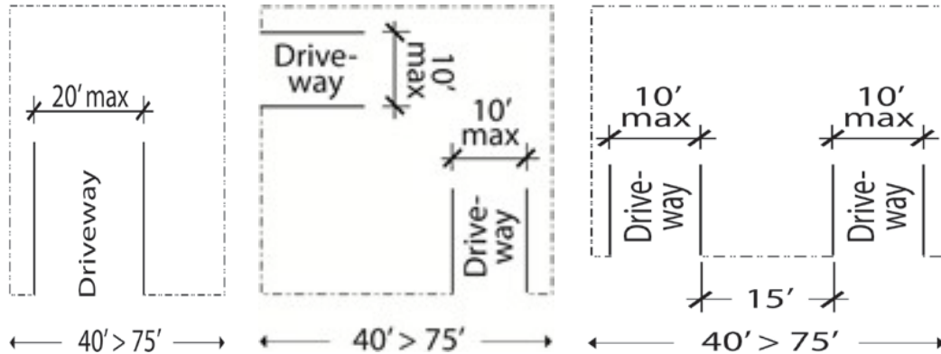
Figure 7:17.4. Driveway Access on Lots at 40 to 75 Feet Wide
