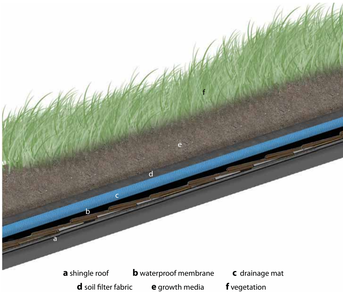
Figure 47: Schematic Section of a Slanted Green Roof
