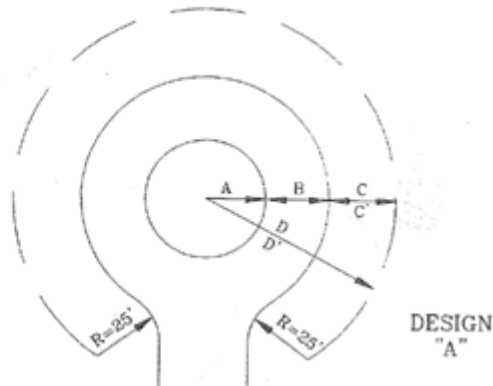
Figure 7:13.1. Typical Cul-de-Sac
