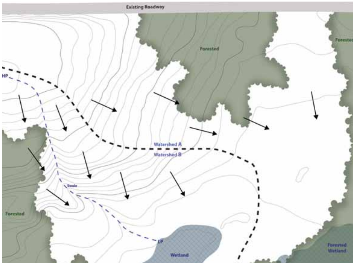
Figure 9: Step 1, Existing Watersheds and Surface Hydrology Map
