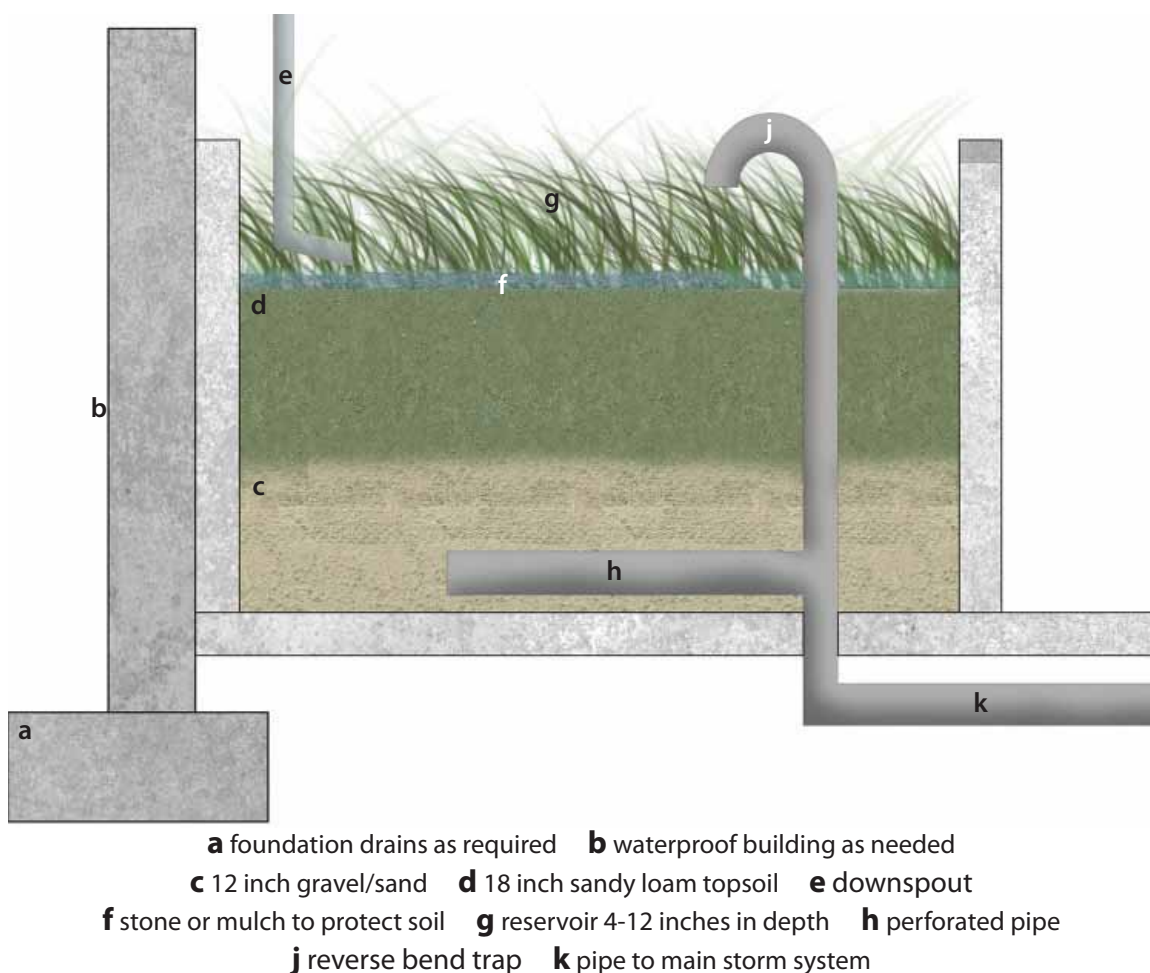
Figure 41: Schematic Section of a Impermeable Stormwater Planter
