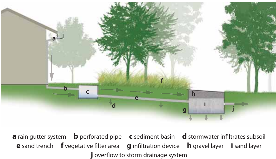
Figure 37: Schematic Section of an Infiltration Device
