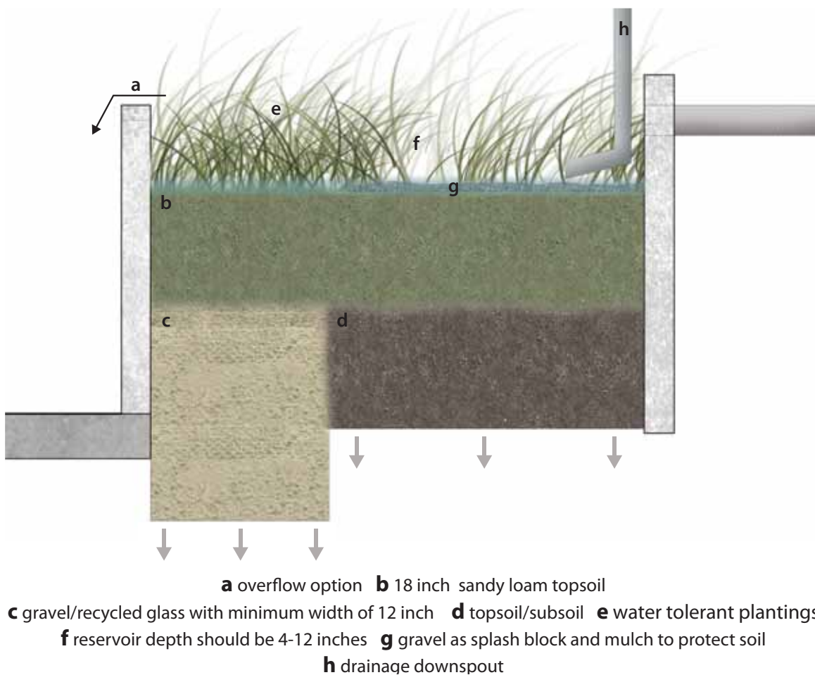
Figure 40: Schematic Section of a Permeable Stormwater Planter
