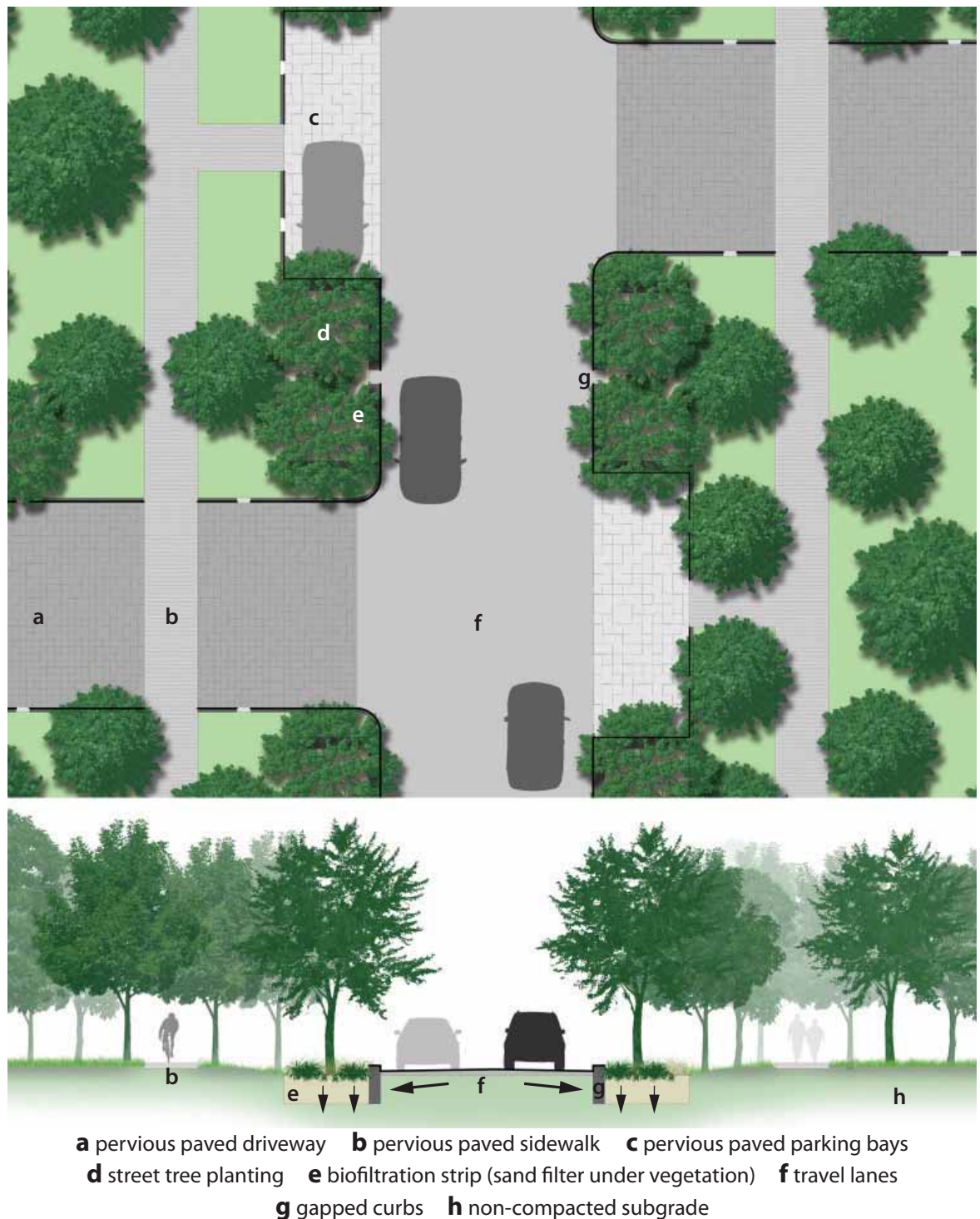
Figure 15: Above, plan of a typical roadway biofiltration strip Below, section of a typical roadway biofiltration strip
