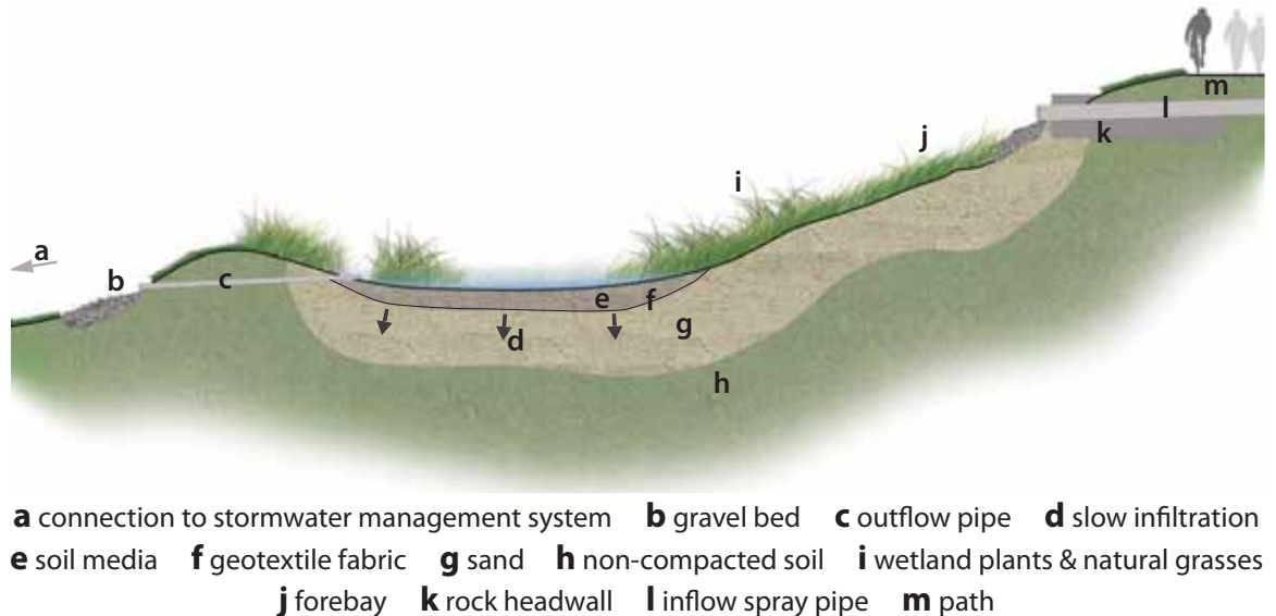
Figure 31: Schematic Section of a Dry Pond
