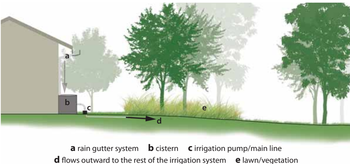
Figure 38: Schematic Section of a Cistern
