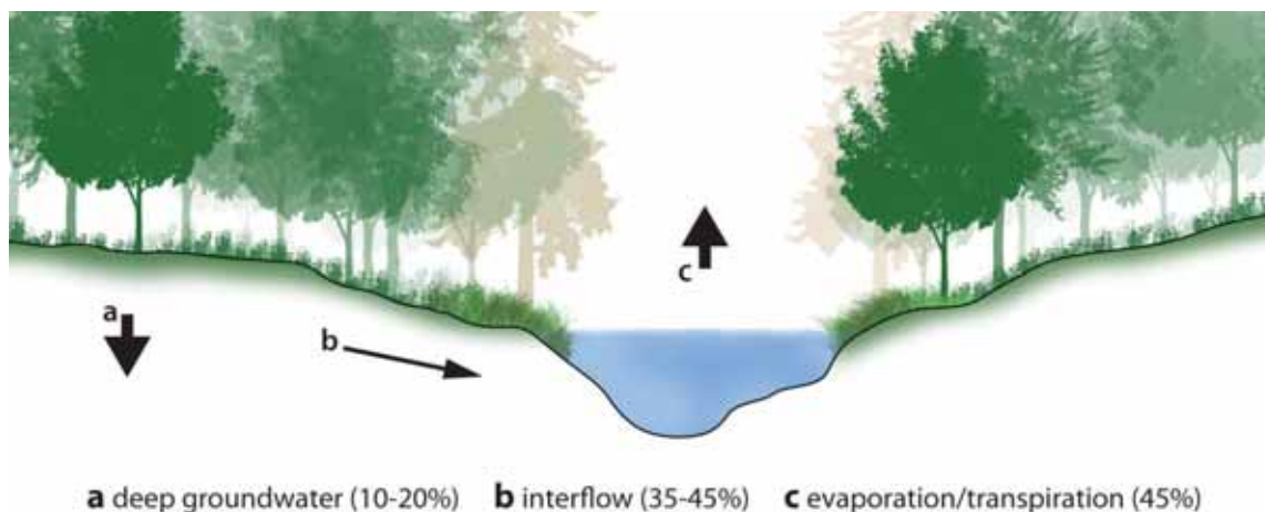
Figure 1: Hydrologic Cycle, Natural Environment
