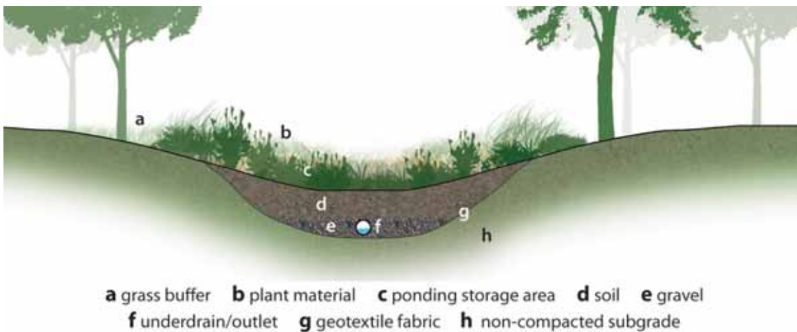
Figure 45: Schematic Section of a Rain Garden
