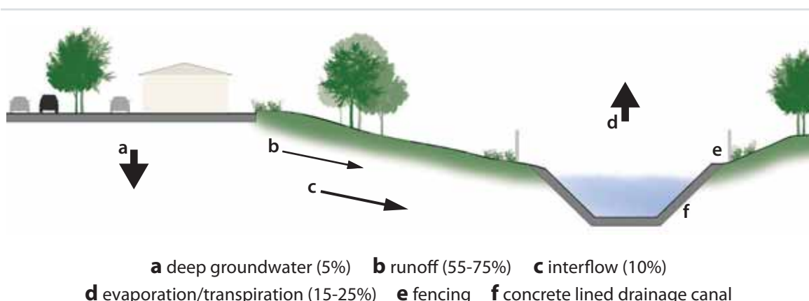
Figure 3: Hydrologic Cycle, Typical Manmade Environment
