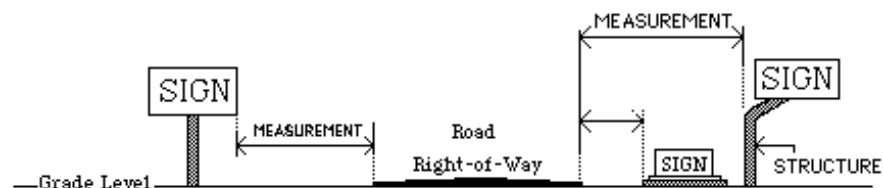
Figure 7:19.2.5.D. Sign Setback Illustration
