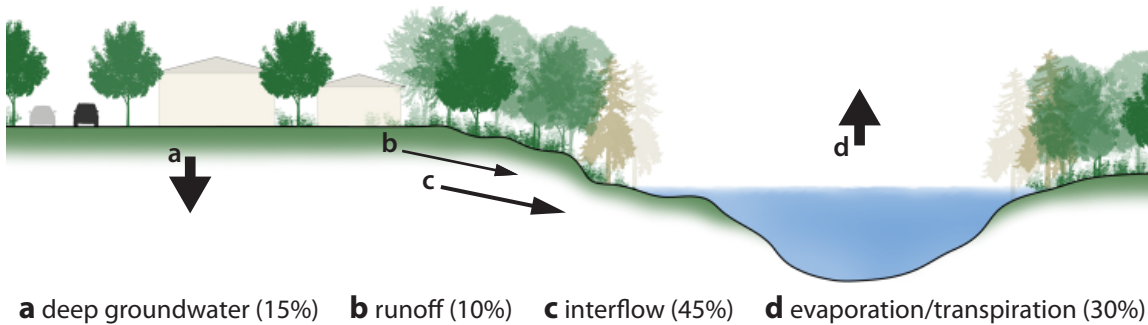
Figure 5: Hydrologic Cycle, Green Environment
