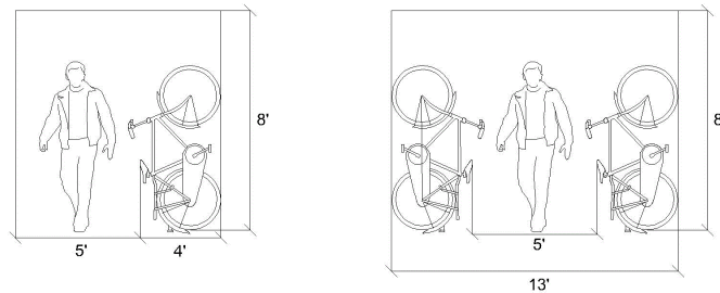
Figure 7:17.8. Minimum Maneuverability Criteria for Vertical Racks
