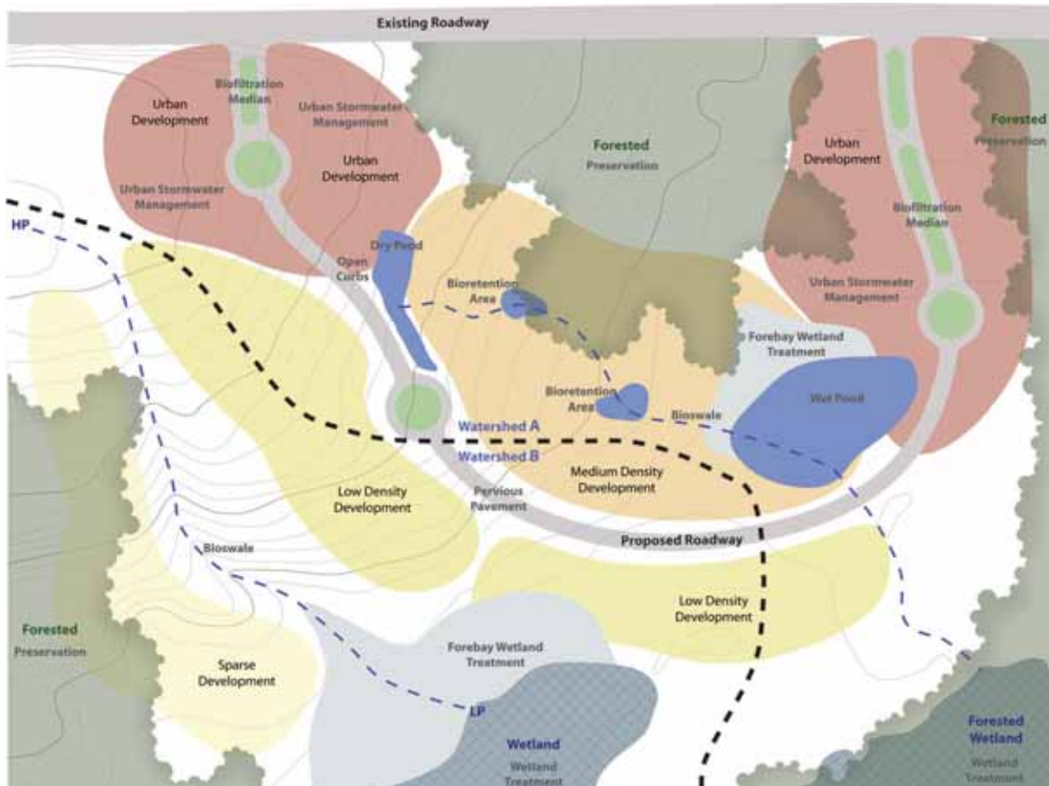
Figure 10: Step 2, Schematic Water Quality Treatment Plan
