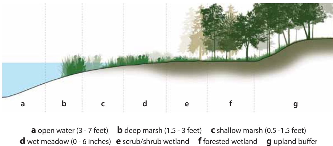
Figure 44: Schematic Section of a Water Quality Wetland
