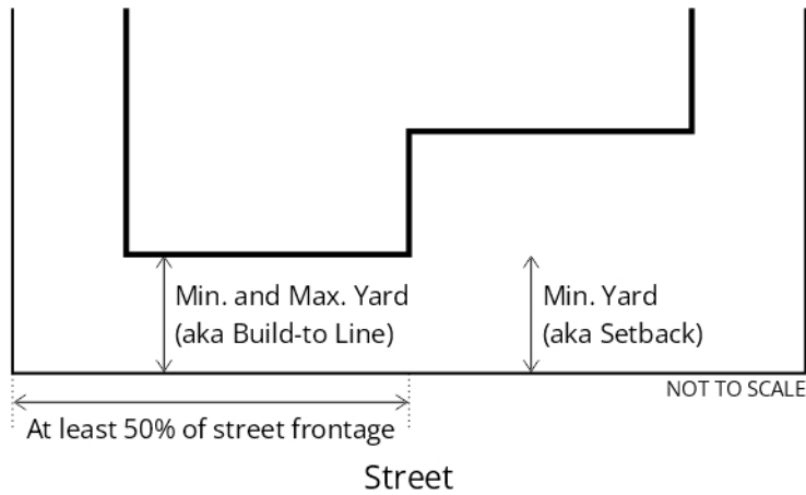
Figure 7:10.1.1.E. Nonresidential Build-To Line
