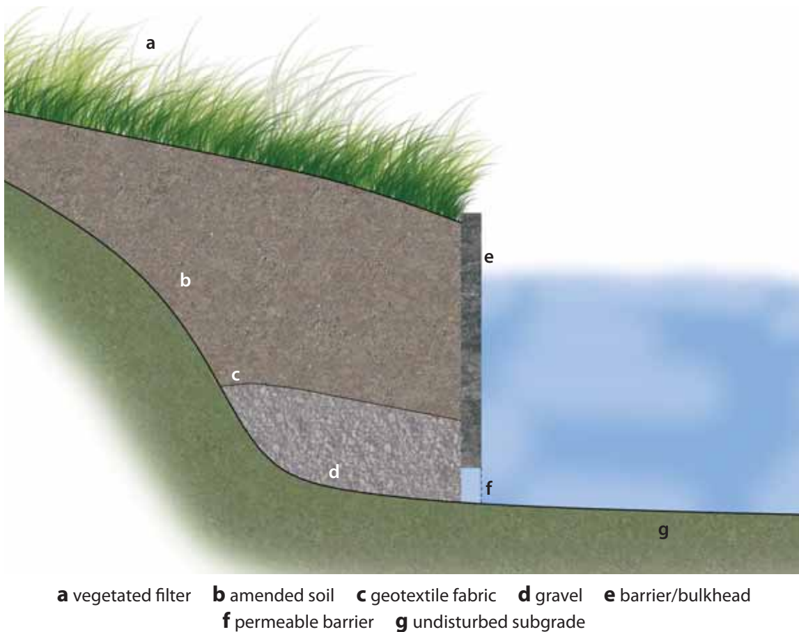
Figure 33: Schematic Section of Bulkhead
