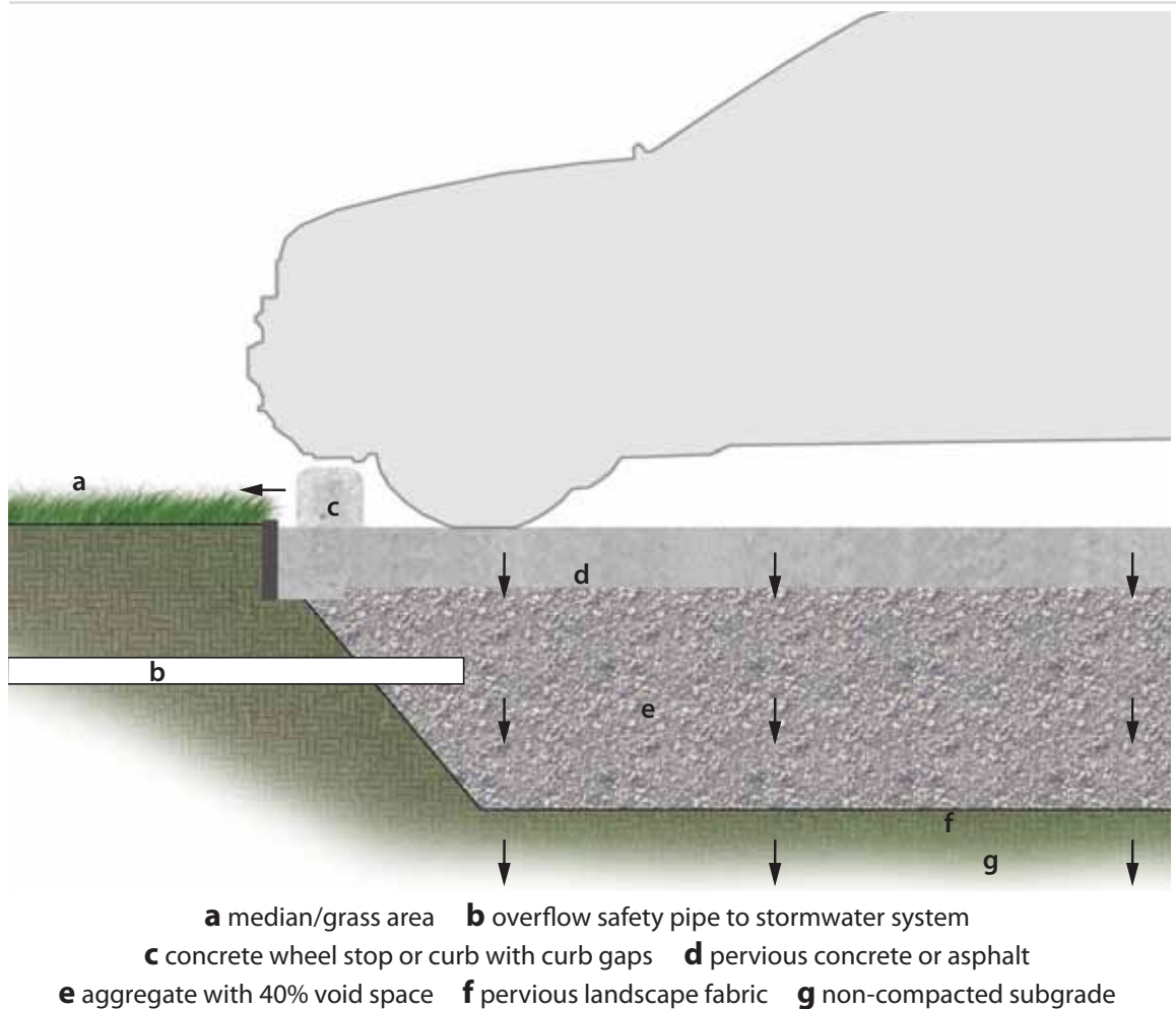
Figure 36: Schematic Section of Pervious Paving with Aggregate Subsurface Storage
