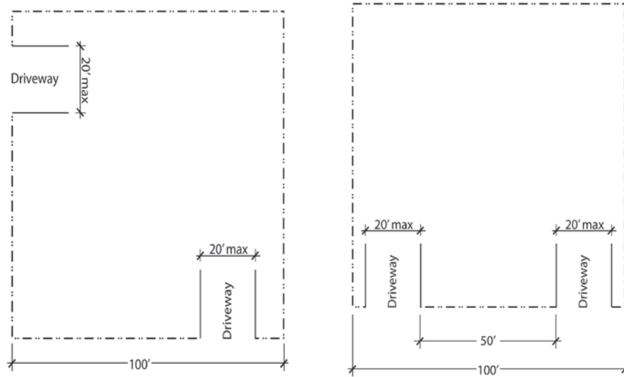
Figure 7:17.2. Driveway Access on Lots at Least 100 Feet Wide
