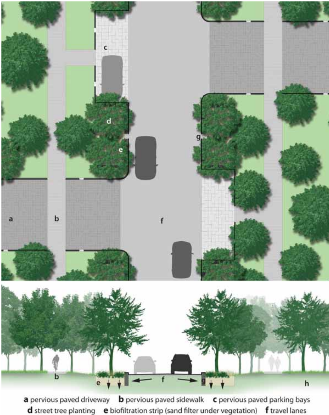
Figure 14: Above, plan of a typical biofiltration median Below, section of a typical biofiltration median
