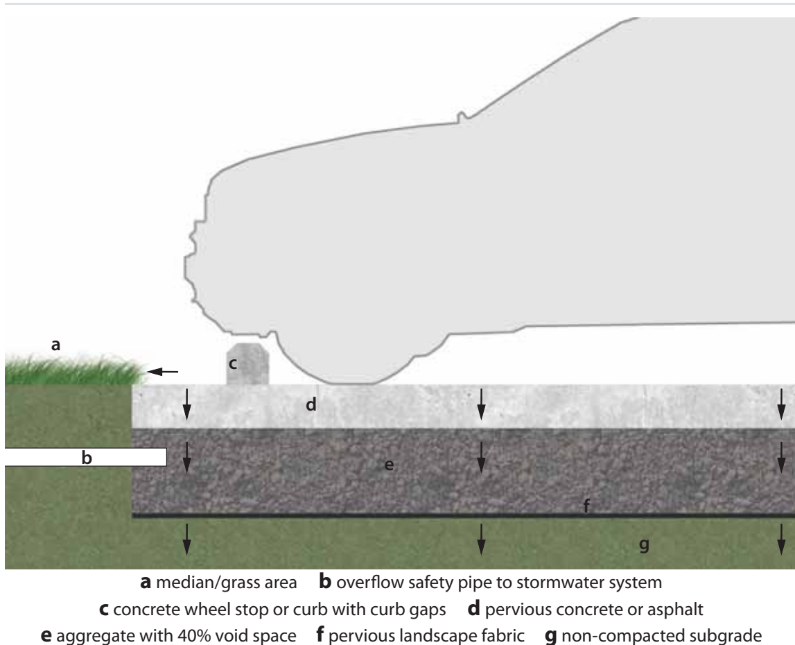
Figure 35: Schematic Section of Pervious Paving
