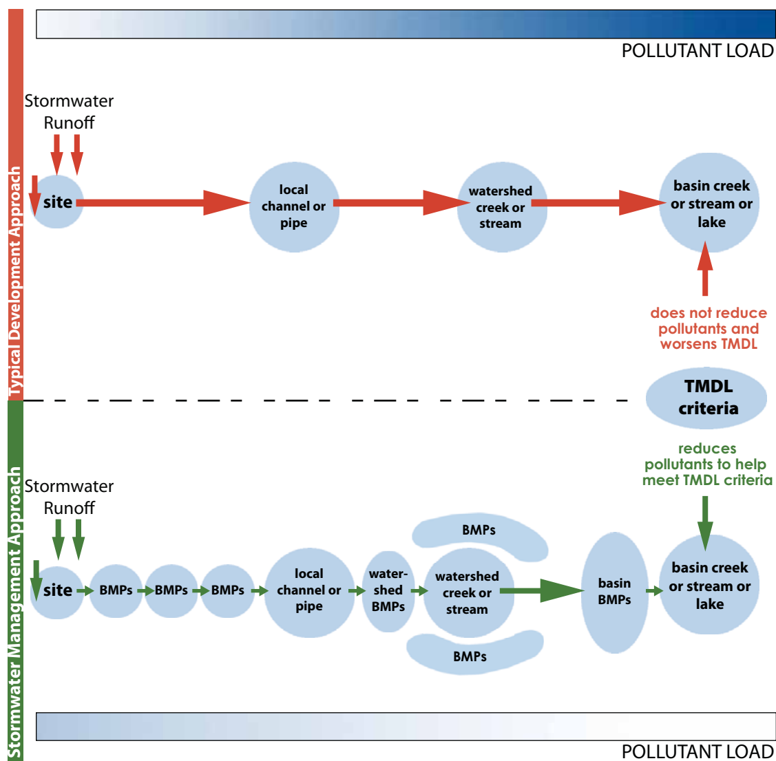
Figure 4: Development Stormwater Treatment Train
