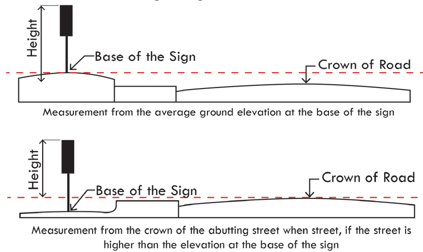
Figure 7:19.2.5.C. Sign Height Illustration
