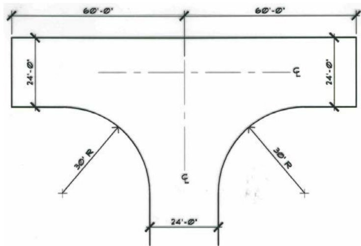
Figure 7:13.2. Typical Turnaround
