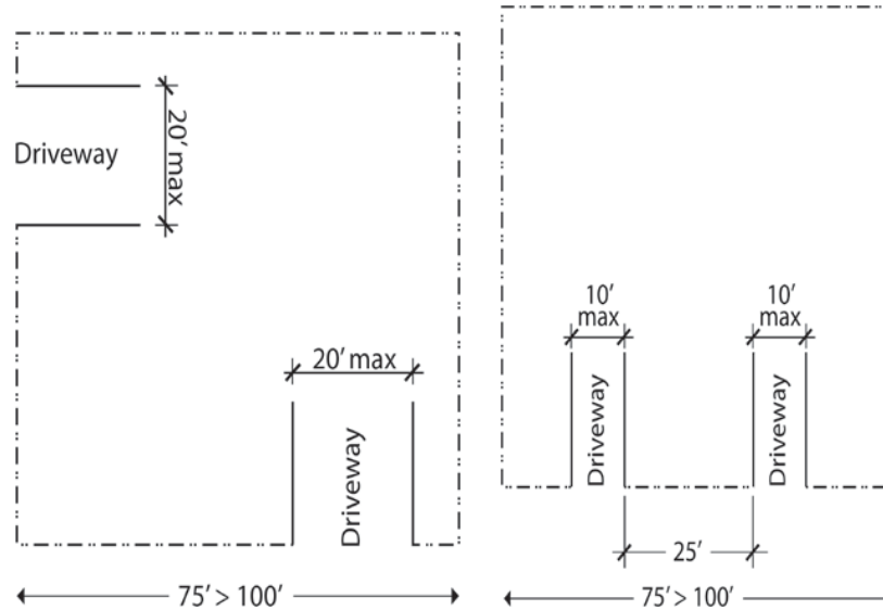
Figure 7:17.3. Driveway Access on Lots at 75 to 100 Feet Wide
