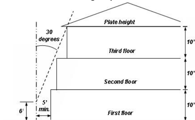
Figure 7:10.1.1.C. Building Stepbacks
